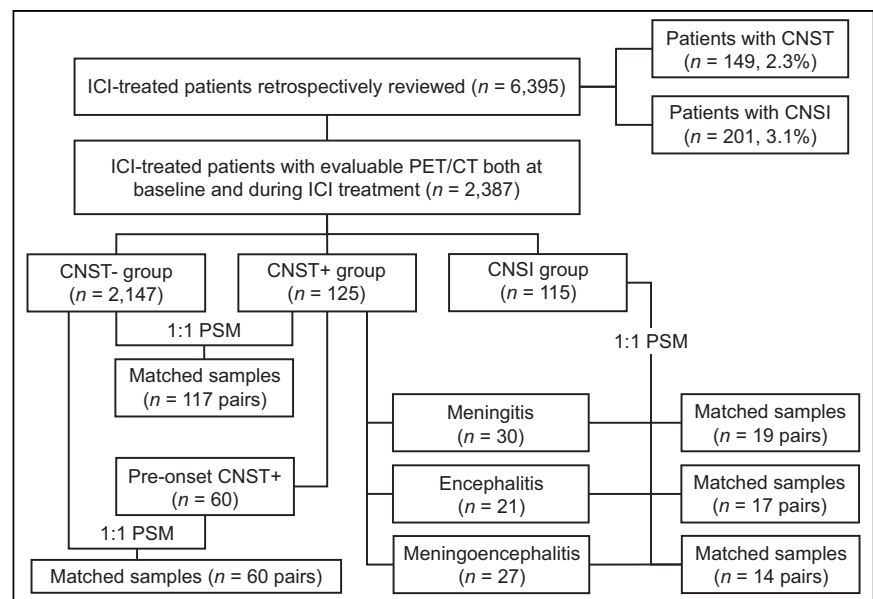
FIGURE 1. Research flowchart.
